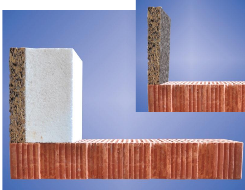
adhesive system insulated (big picture); adhesive system standard (small picture)
